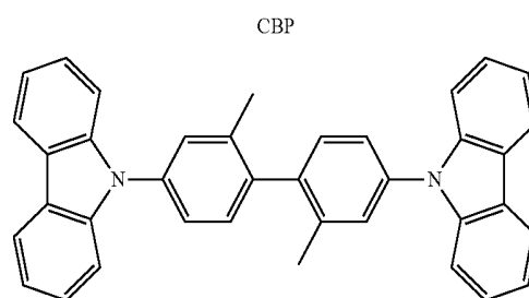
dmCBP
