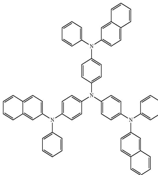
2-TNATA
